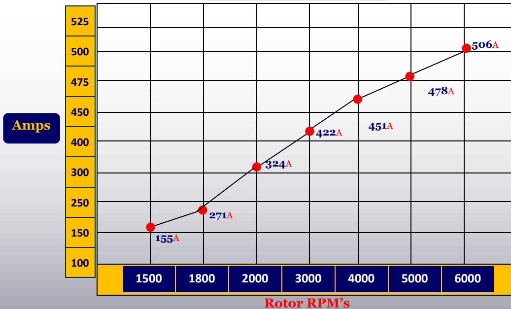
Alternator Output
