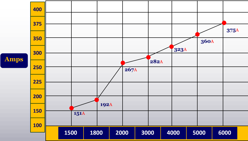
Alternator Output
