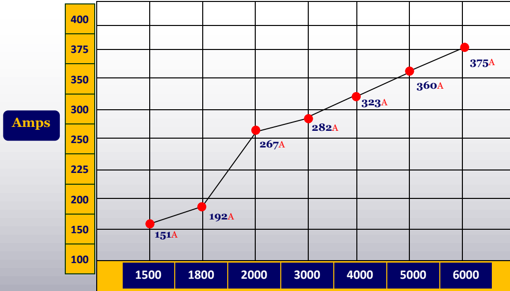
Alternator Output
